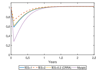
Fig. 4. Alternative preference parameters. We plot the optimal response to volatility shocks as we change the IES from 0.2 (the CRRA case) to 1 (our benchmark case) to 2. The top panel does this for our baseline model parameters, while the bottom panel does this for the case in which we allow changes in volatility to affect the discount rate share.
